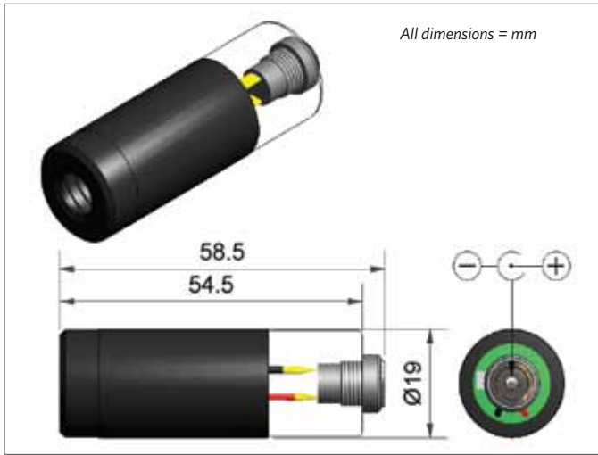
DC Jack
