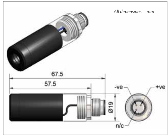
Screw Connector
