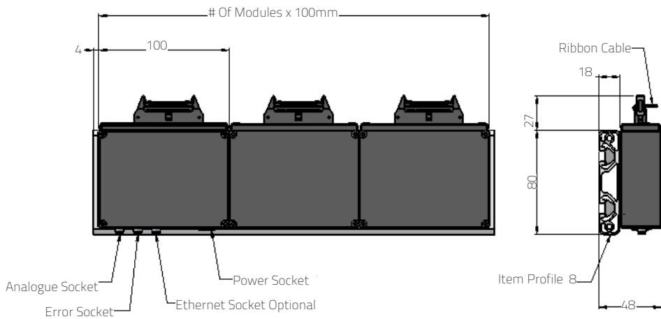
Electronics Module Mounting Option 1
