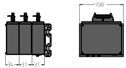
Electronics Module Mounting Option 3
